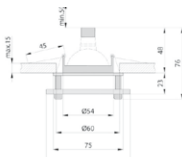
Rozetna DL-20s MR 16, 12V, aluminium
